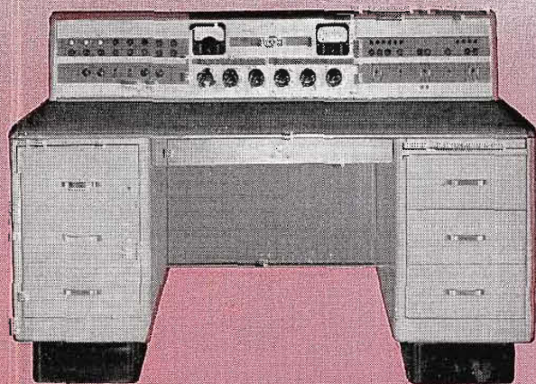
CONTROL CONSOLE contains controls for both the transmitter and audio channels. Every major function of the transmitter is at the engineer's finger tips or within easy viewing distance.
