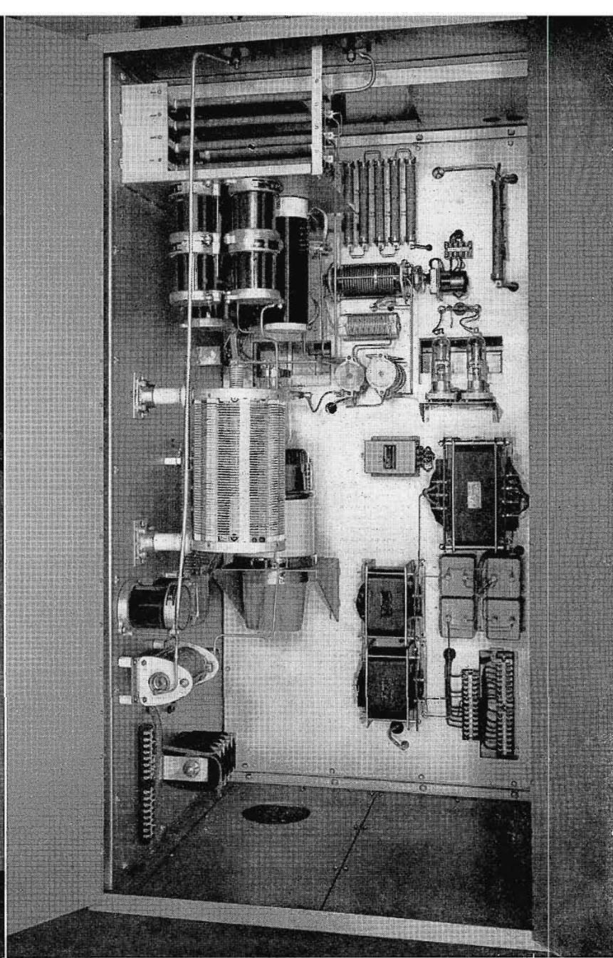
FIG. 6. The intermediate power amplifier circuits are located in the rear of the exciter cubicle. Note the accessibility of all components and wiring connections.
