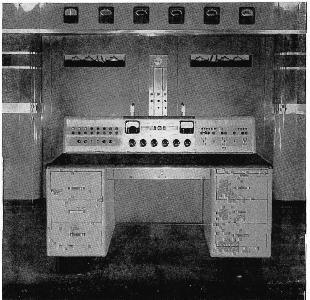
FIG. 1. (Above) The streamlined, unified front of the 50-F contains wide, full-length doors which provide direct, non-hampered access to the low-power r-f modulator and power amplifier compartments. The door at the right is the entrance to the non-interlocked area which contains the control and distribution unit and the main switchboard unit (see diagram on following page).
