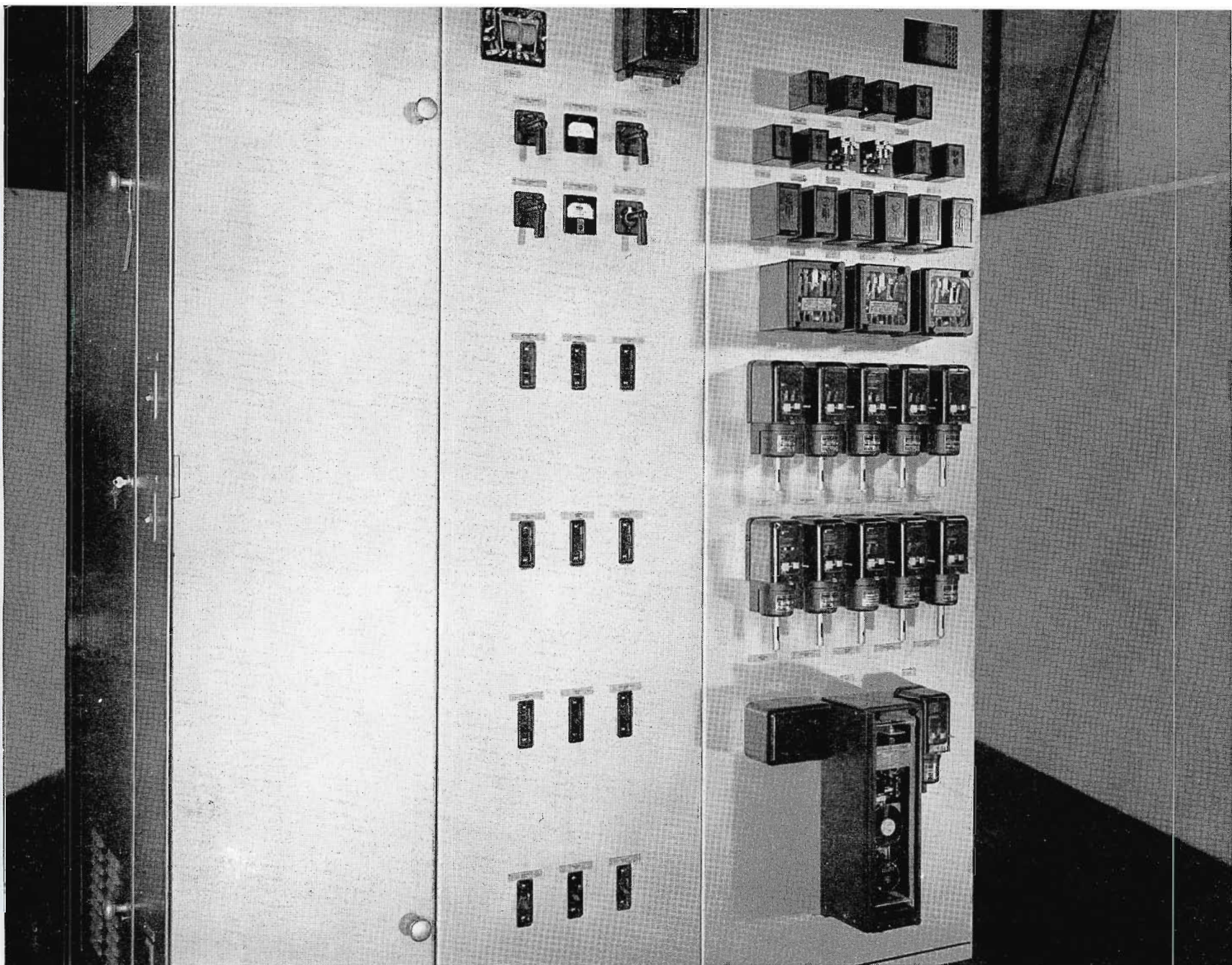
FIG. 11. All time delay relays, overload relays and distribution circuit controls are mounted on the control and distribution unit which is located just inside the righthand door of the transmitter. This is a totally inclosed unit which is designed, manufactured, and assembled according to best switchgear practice. The BTA-50F includes more advanced and more complete protective and control circuits than any transmitter designed to date.
