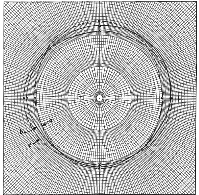
FIG. 7. Patterns obtained when parallel length P was shortened. Curve a is for same length as Curve c of Figure 6. Curve b is for A = 26'' and P = 27'' . Curve c is for A = 26'' and P = 28'' .
