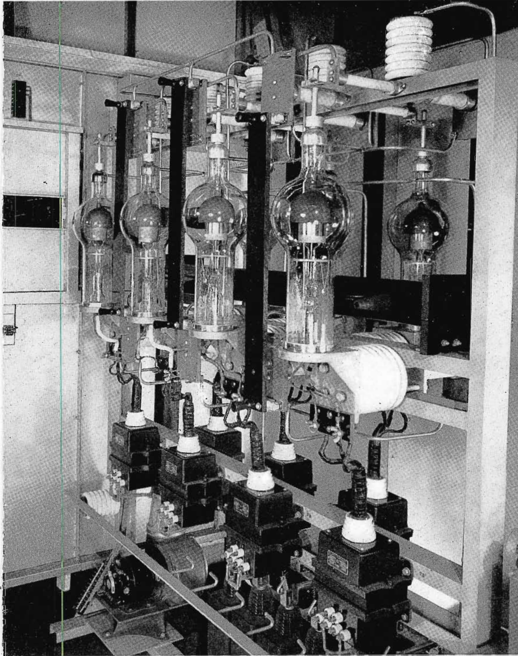
FIG. 12. The high-voltage rectifier of the BTA-50F uses six RCA-857B's in a three-phase, full-wave circuit. A seventh tube—maintained at operating temperature at all times—may be quickly switched into the circuit whenever any of the six operating tubes becomes defective.
