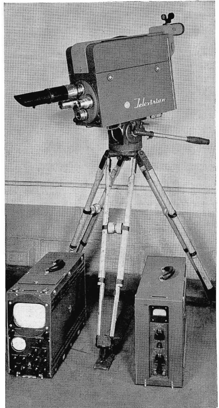
FIG. 5. (Above) Illustrated here is a complete Type TK-30A Camera Equipment. This grouping, often referred to as a "camera chain," is a complete operating unit in itself (except that it must receive synch signal from an external source). When a three-camera setup is desired the equipment units shown above must be added to the equipment grouping shown in Figure 1. For a four-camera setup, two complete groupings, as shown above, must be added.
