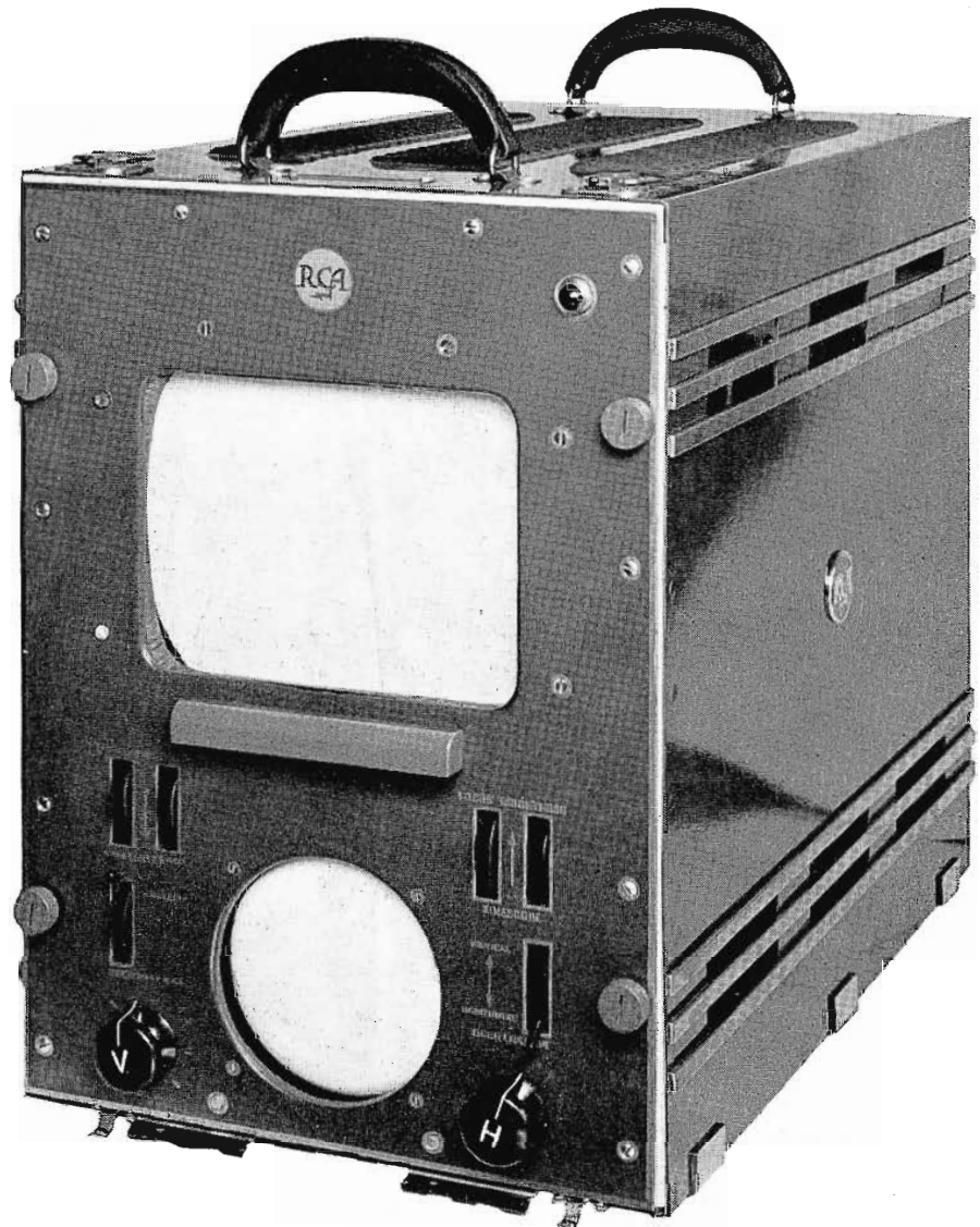
FIG. 13. The TM-5A Master Monitor mounted in a field carrying case is shown here. This unit, the chassis of which is identical with that of console and rack-type monitors, makes use of a 10-inch kinescope and hence requires a somewhat larger case than the other units. It obtains required operating voltages from the power supply unit used with the TS-30A Switching System.
