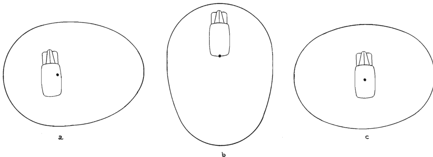
FIG. 4. Patterns made with the antenna mounted at different positions on the car roof show the effect of the car body on the reception patterns. This may be compensated by changing the ratio of dimensions as described in the text.
