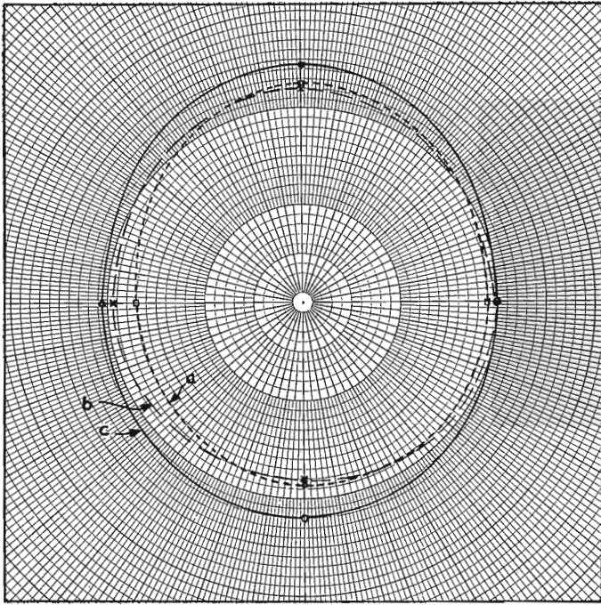
FIG. 6. Patterns obtained with antenna arrangement shown in Figure 5. Curve a for A = 26'' and P = 30'' . Curve b for A = 26'' , P = 29'' . Curve c, same as b, but antenna moved toward rear of car.
