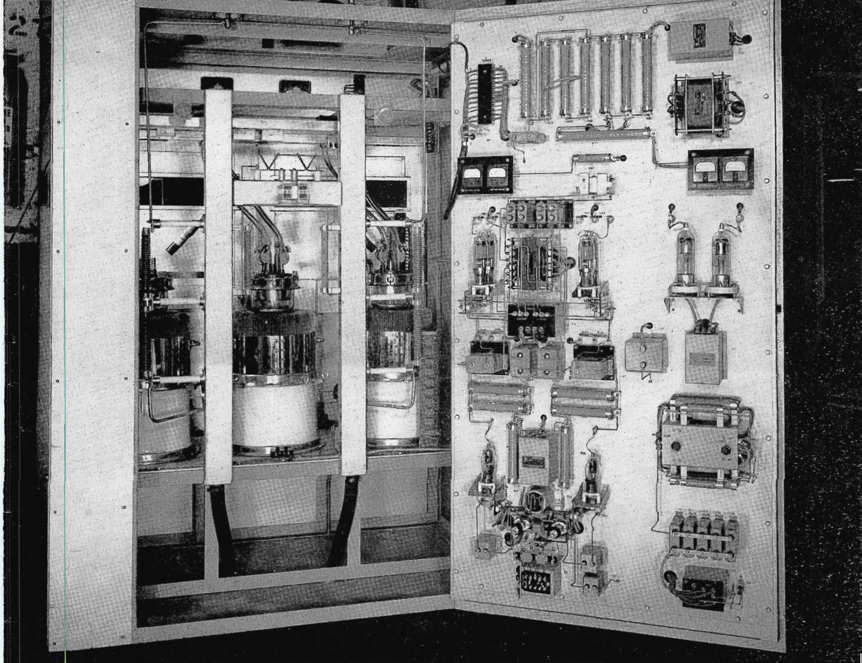
FIG. 10. Rear view of the audio and modulator compartment. All of the low-power audio components are mounted on the inside of the rear door—making them easily accessible for inspection and maintenance. Use of cathode-follower circuits in the driver stage provides a number of advantages over older type drive circuits.
