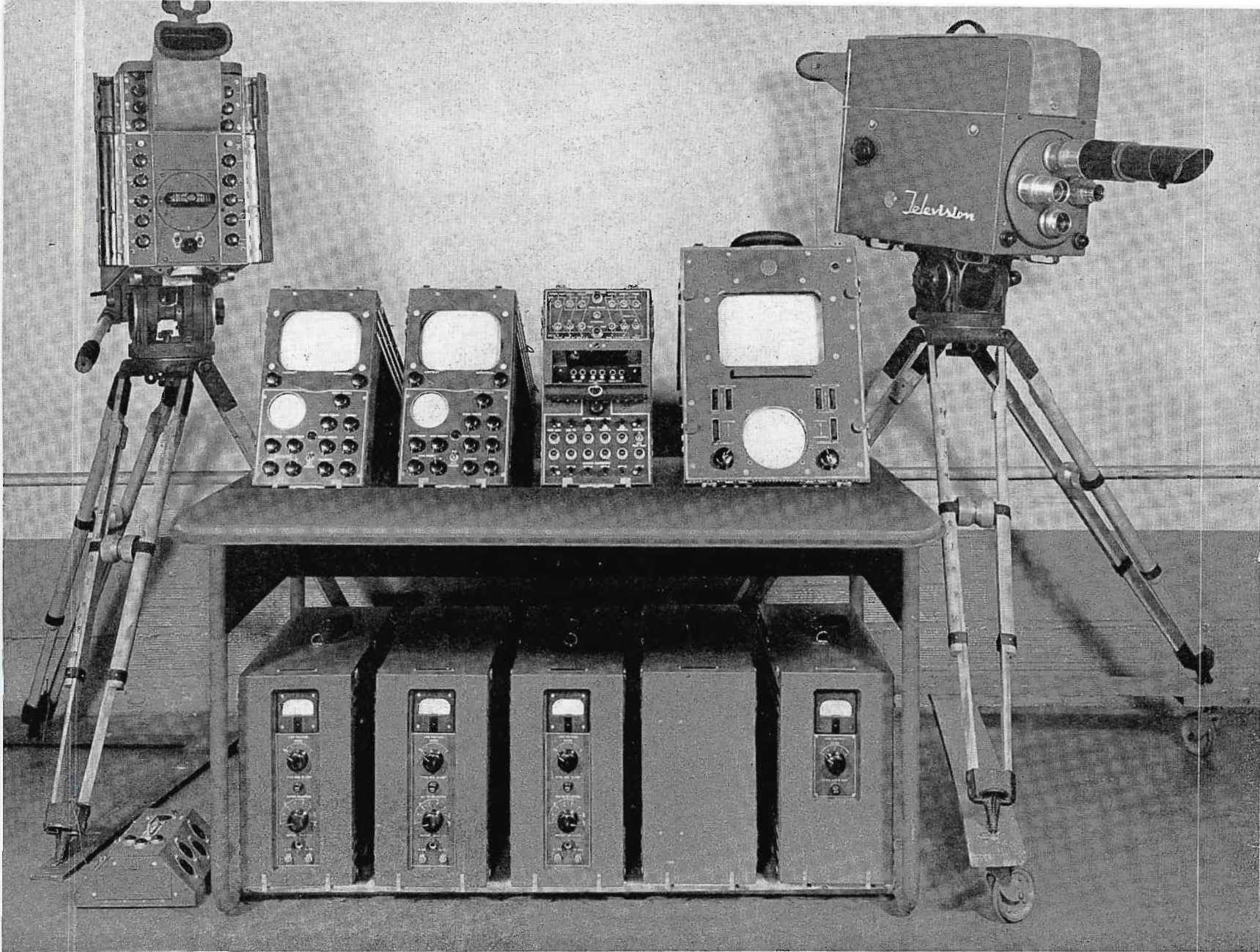
FIG. 1. (Above) This is a complete two-camera field equipment (less cables) set up on the special field control desk. The two Image Orthicon cameras, with built-in electronic viewfinders, are shown at the left and right of the desk. The camera at the left has the rear control doors open to show position of minor controls used in making initial adjustments. The units on the desk are, left to right, Camera Control No. 1, Camera Control No. 2, Switcher and Master Monitor. Those under the desk are, left to right, Power Supply for Camera No. 1, Power Supply for Camera No. 2, Power Supply for Switcher and Monitor, and the two units containing the Synchronizing Generator. On the floor, at the left of the table, is the junction box for a-c power connections. Not shown are the interconnecting and camera cables, which are also furnished.
