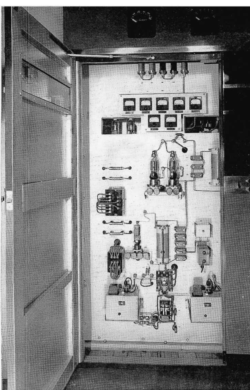
FIG. 5. Low-power r-f stages are located on a vertical panel in the front of the exciter cubicle. Duplicate oscillators are provided, with manual or automatic changeover being available.
