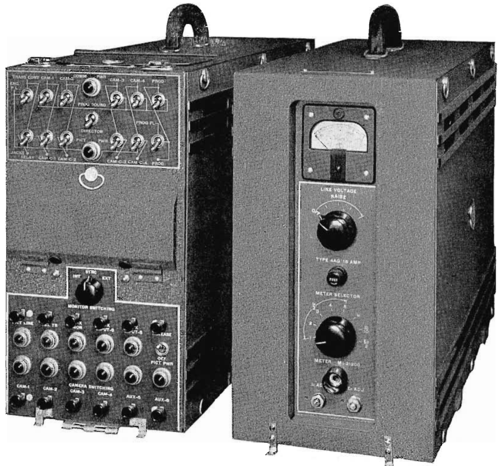
— FIG. 11. The TS-30A Field Switching Equipment consists of the switcher (left) and a standard power supply unit, which also furnishes all voltages required for operation of a TM-5A Monitor Unit.
