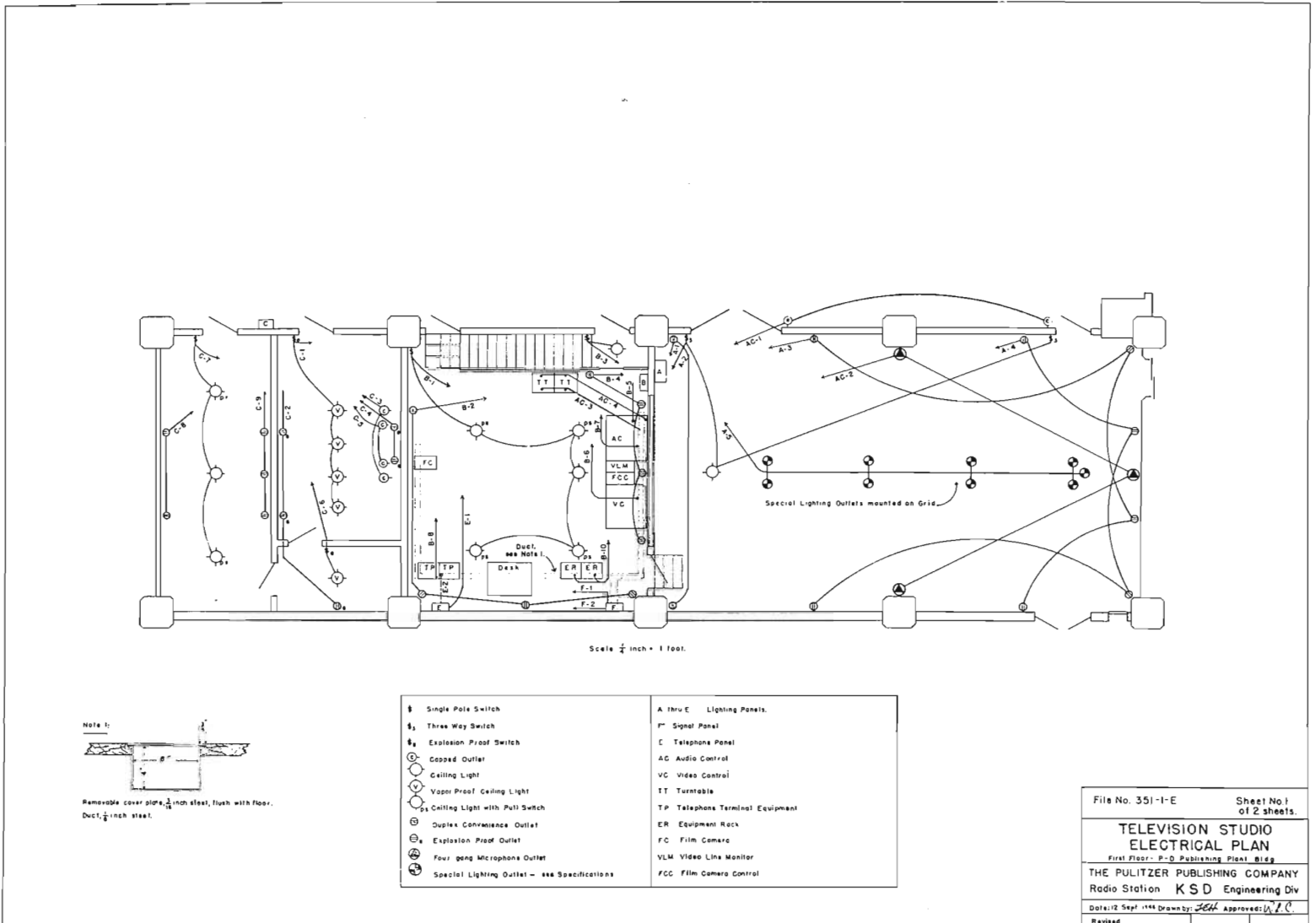
FIG. 7. Floor layout of KSD-TV's temporary setup showing, left to right, the workshop, telefilm room, control room, and studio proper. Location of main equipment items, outlets, and connections is indicated by symbols which are identified in the legend.
