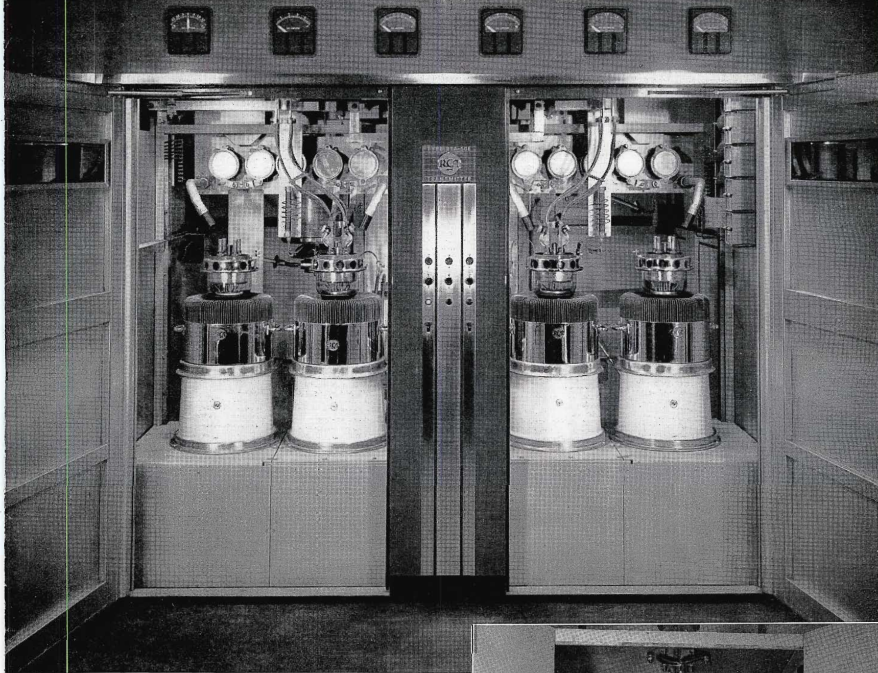
FIG. 7. (Above) Two large doors provide access to the front of the power amplifier compartment. Four tube positions are provided, two of which are for spare tubes. Placing a spare tube in the circuits is easily accomplished by moving flexible filament and grid leads.
