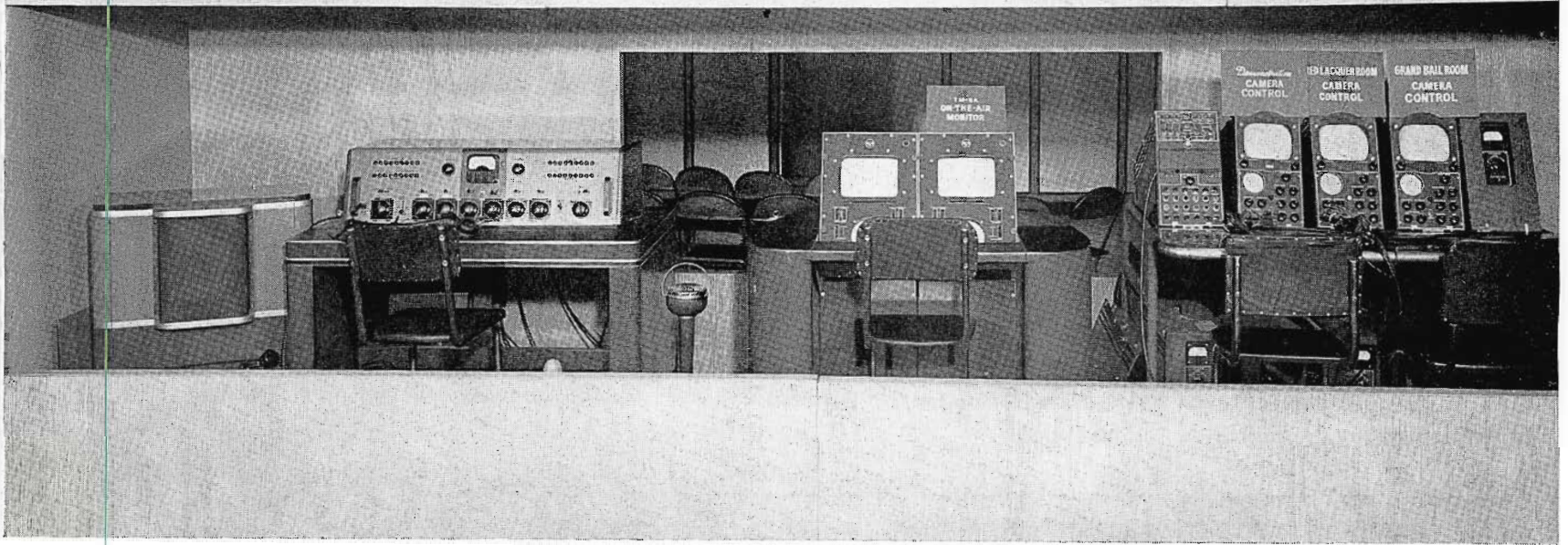
FIG. 5. Closeup of television control equipment showing (left to right) monitoring loudspeaker, audio console, on-the-air and film monitors, and portable camera control equipment. "Window" at rear looks into television "overflow" room.
