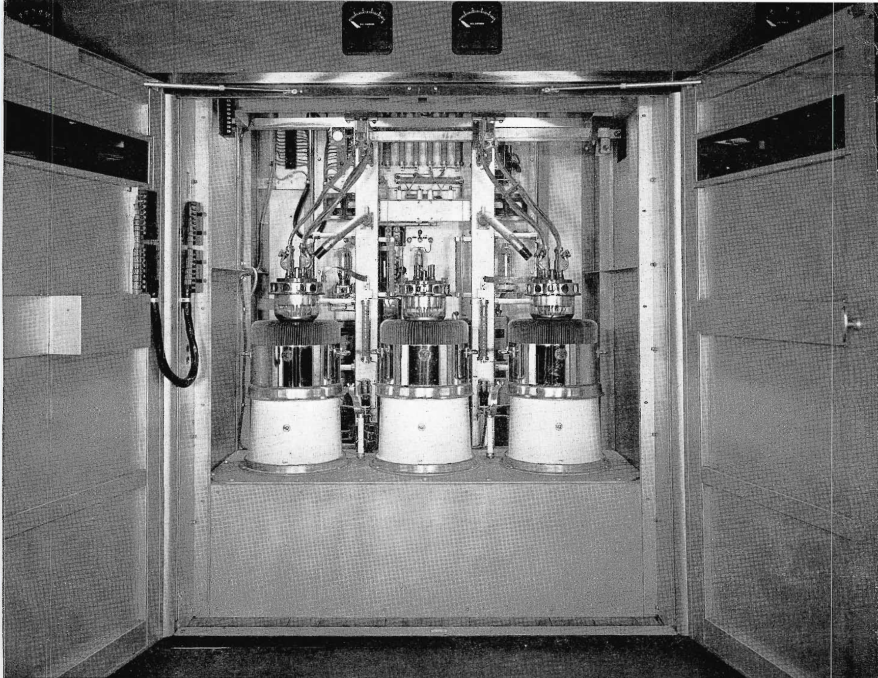
FIG. 9. Front view of the audio and modulator compartment. Three tube positions are provided, the center being for a spare tube which can be inserted in place of either modulator simply by moving the flexible grid and filament connectors. This arrangement greatly reduces the time lost in case of a tube failure.
