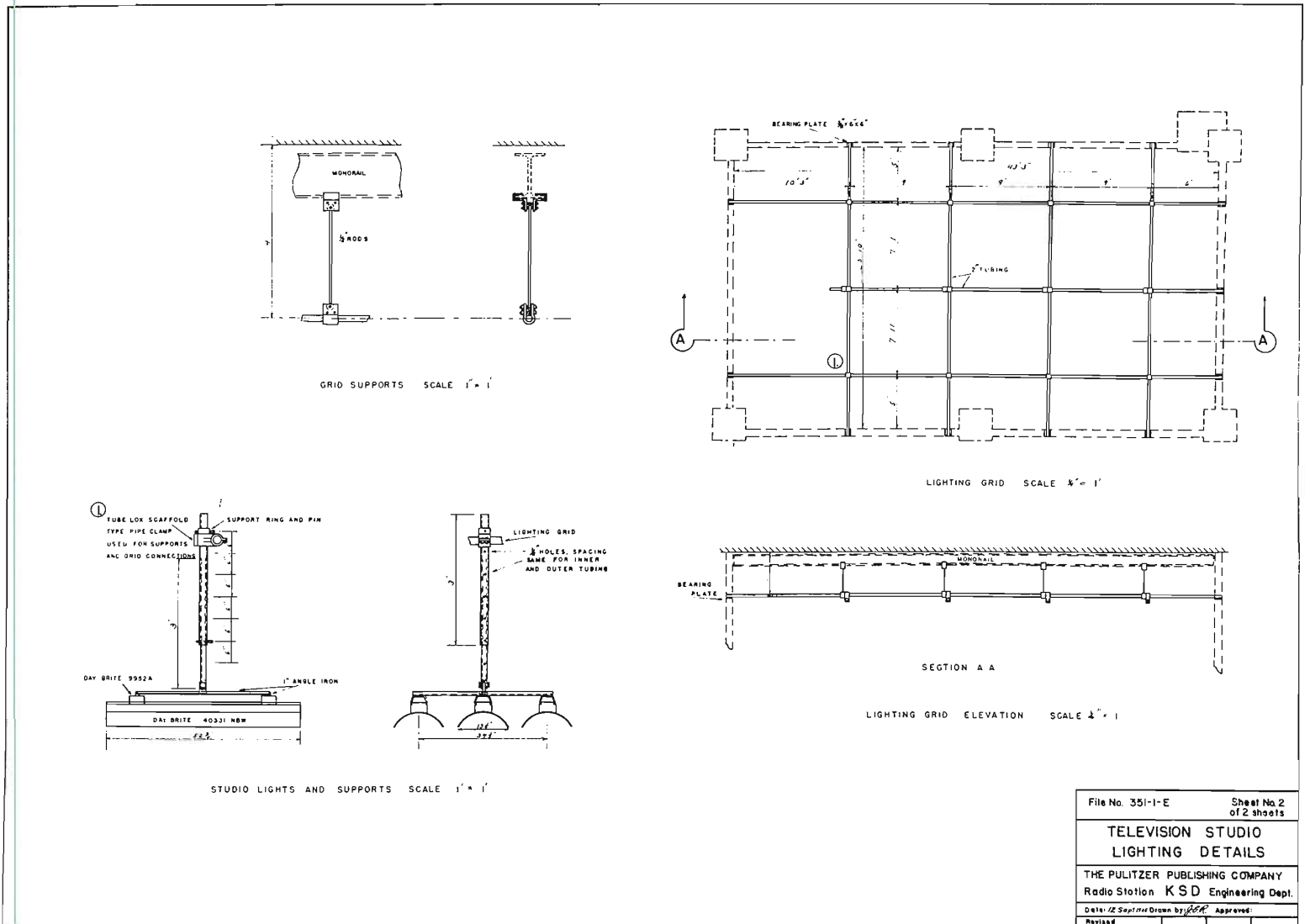
FIG. 8. Construction details of the overhead light banks and iron-pipe grill which is used to support them. Light banks were assembled from available commercial-type fluorescent fixtures. They can be detached quickly from the grill and moved about as desired.
