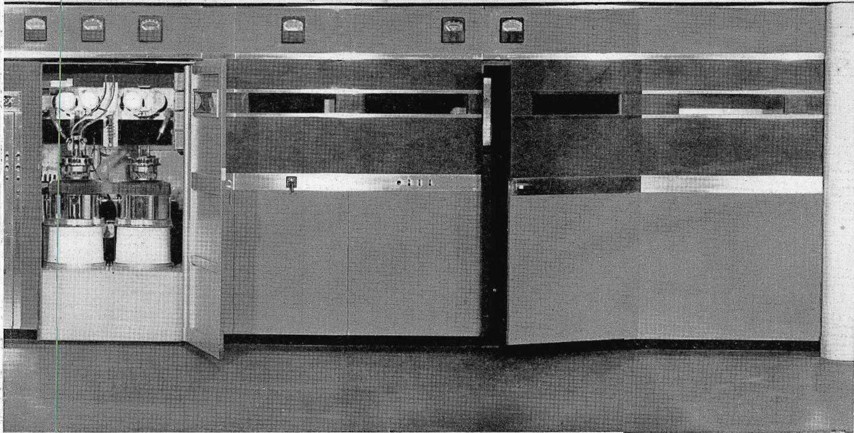
FIG. 1. (Above) The streamlined, unified front of the 50-F contains wide, full-length doors which provide direct, non-hampered access to the low-power r-f modulator and power amplifier compartments. The door at the right is the entrance to the non-interlocked area which contains the control and distribution unit and the main switchboard unit (see diagram on following page).
