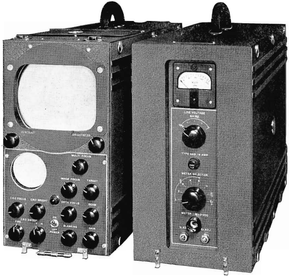
FIG. 7. Camera control unit (left) and power supply unit which furnishes all voltages for the camera control unit and the camera.
